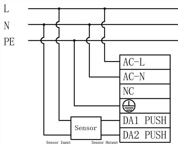
Wiring diagram of corridor dimming
